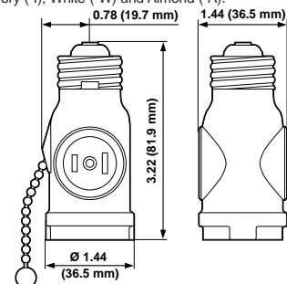
LAMPHOLDER/2 OUTLETS Cat. No. 1406
