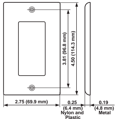
Single-Gang Standard Size Decora Wallplates
